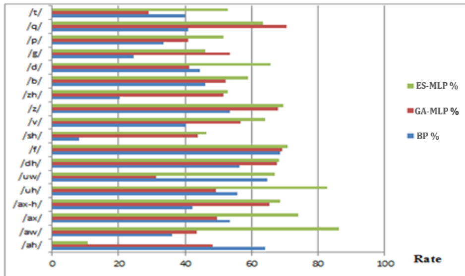
Fig. 4. Recognition scores.
